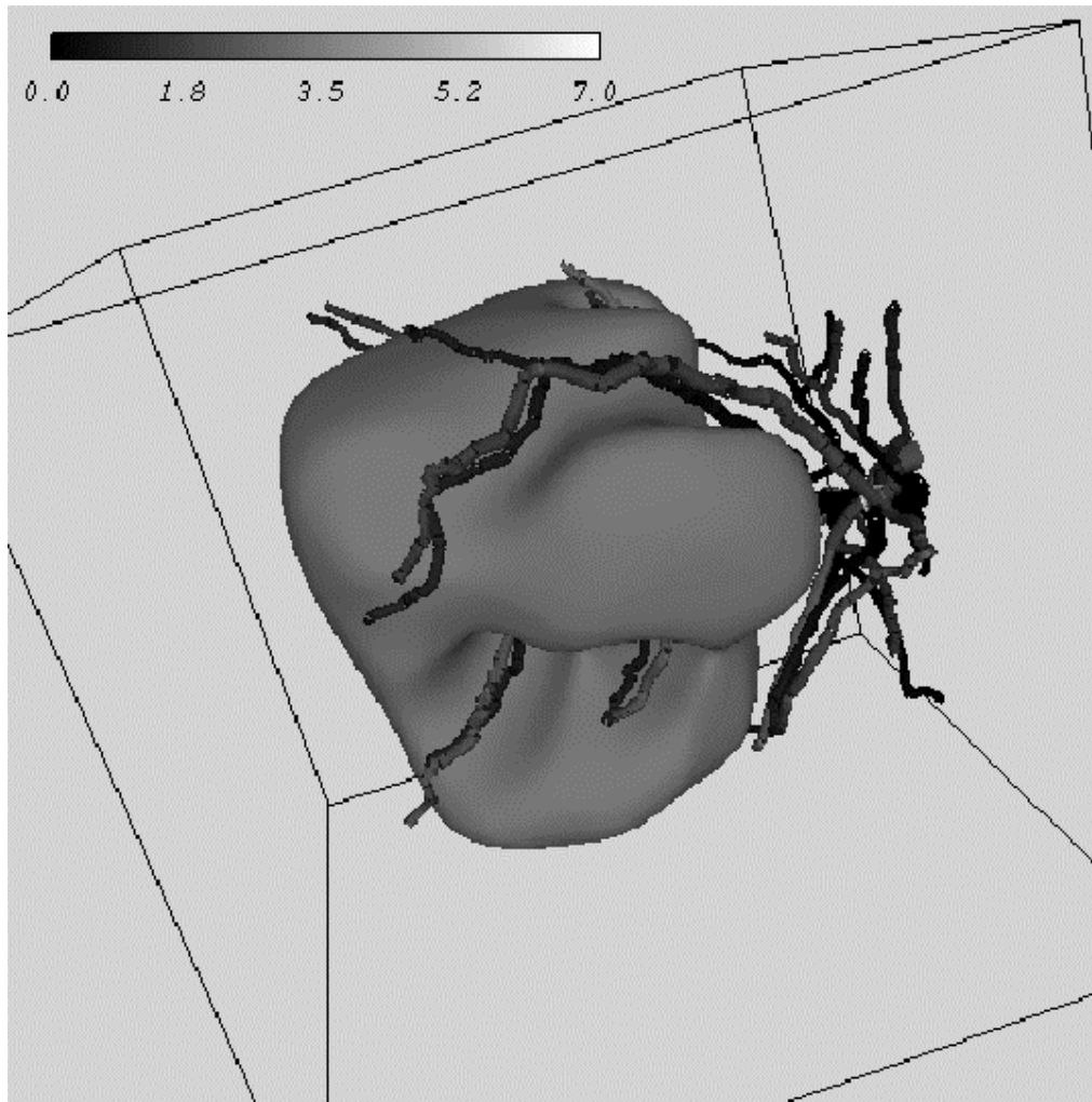
Figure 6: Temperature isosurface for temperature rise of 4 K in a heated tissue cube, in which the detailed artificial vasculature of Figure 5 is reduced to only the larger vessels.
