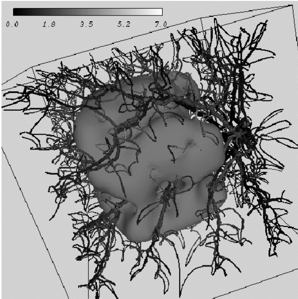
Figure 5: Temperature isosurface for temperature rise of 4 K in a heated tissue cube, in which a detailed artificial vasculature is present. The legend describes the color coding of the vessel blood temperatures in K.
