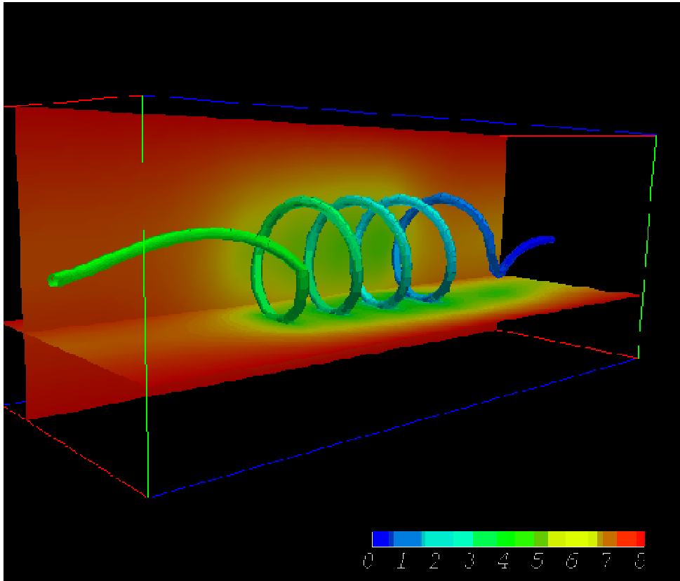
Figure 2: Artificial vessel describing a helix. This geometry was in Chapter 2 used to investigate the accuracy of the model for curved vessels.
