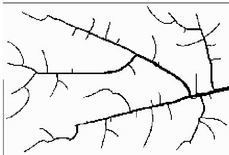
(c) n = 54 , \gamma = -2.0 , \beta = -1 \cdot 10^{-6}
