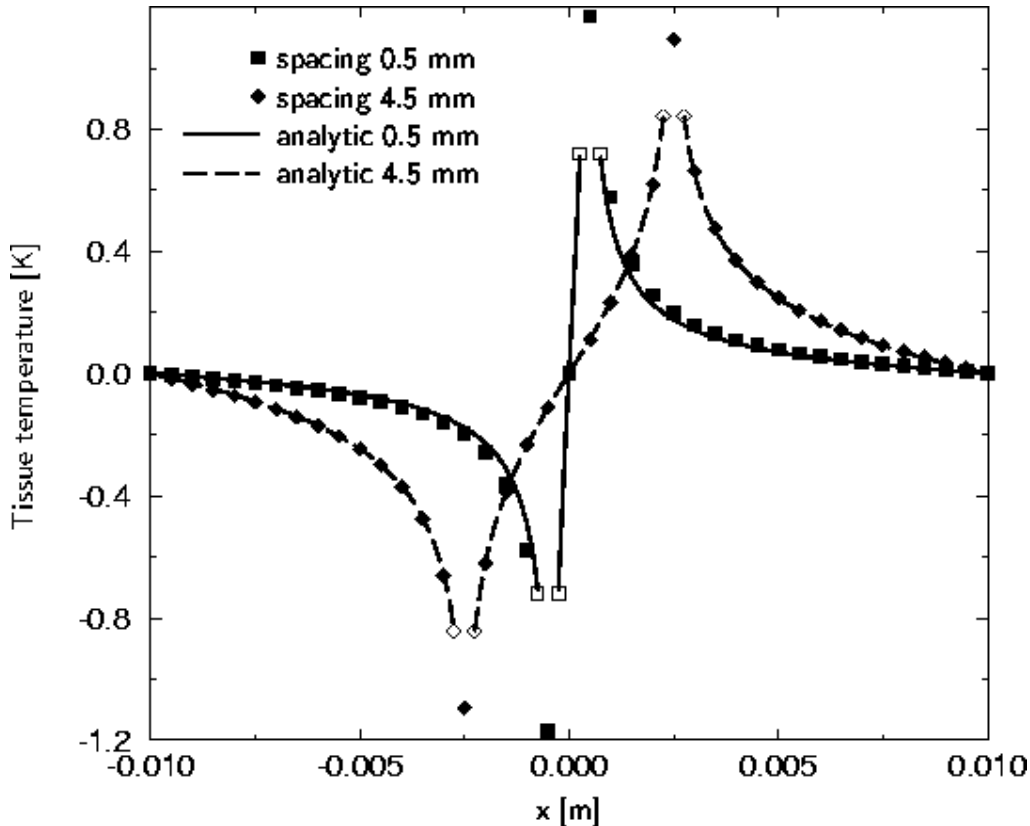
Figure 3: Temperature profile on line through two counter current vessels in a tissue cylinder. The wall temperatures according to the program are indicated by open symbols. There is very good agreement between model prediction and analytical results.
