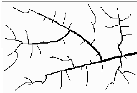
(e) n = 54 , \gamma = -1.5 , \beta = -4 \cdot 10^{-5}
