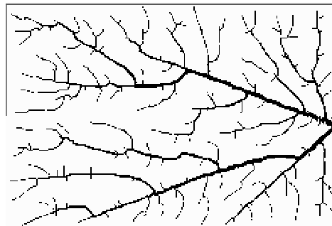
(f) n = 218 , \gamma = -1.5 , \beta = -7 \cdot 10^{-6}
